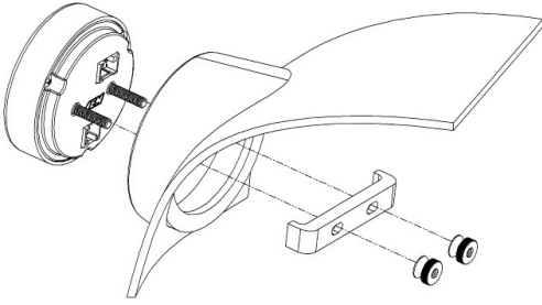
Installation using supplied bracket
