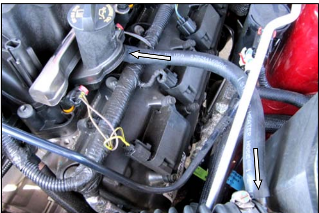
14. On V8 motors, replace the factory crankcase breather line with the 13" Breather Hose (#5) and connect it to the Airaid Intake Tube. Disregard the 90 deg. Elbow (#7) it will not be used.
