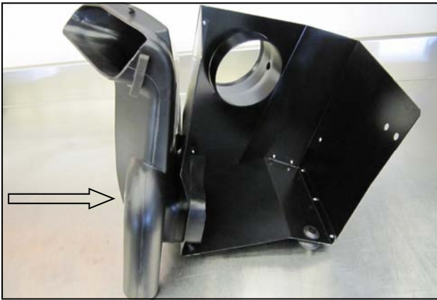
10. Transfer the factory air inlet from the airbox and into the Panel assembly.
