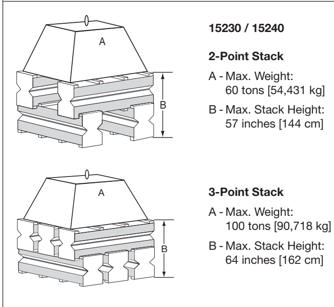
Figure 1, Box Stacking Arrangements (typical).
