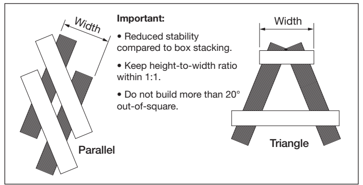
Figure 2, Alternate Stacking Arrangements (typical).
