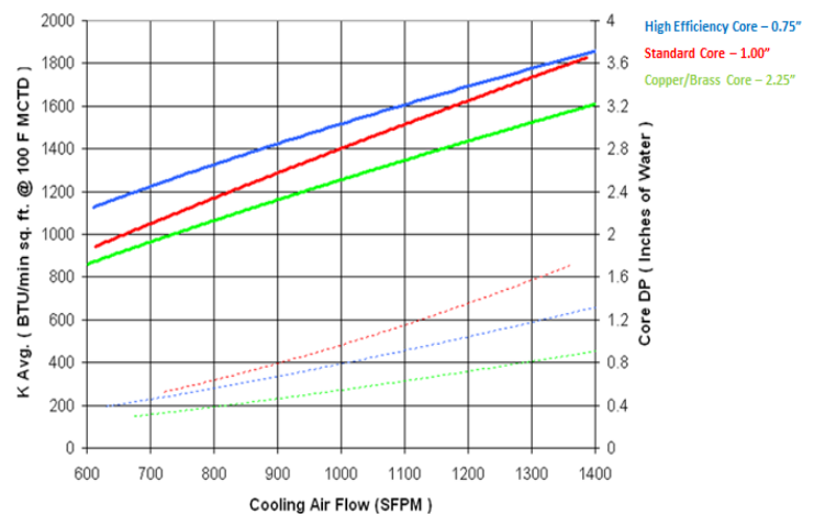
Narrower High Efficiency Core Delivers More Cooling
