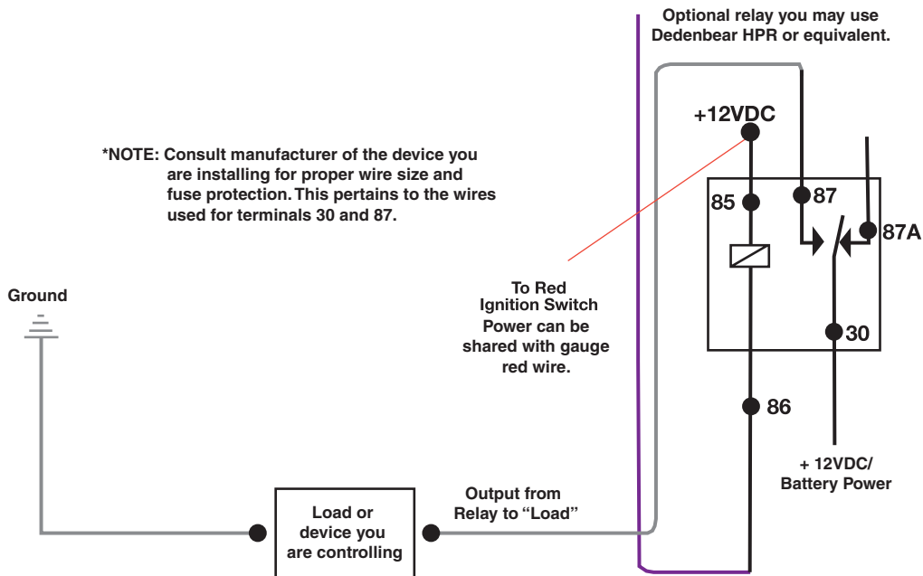
From Gauge Pin 8 Output/Purple to Relay #86 DIAGRAM 2
