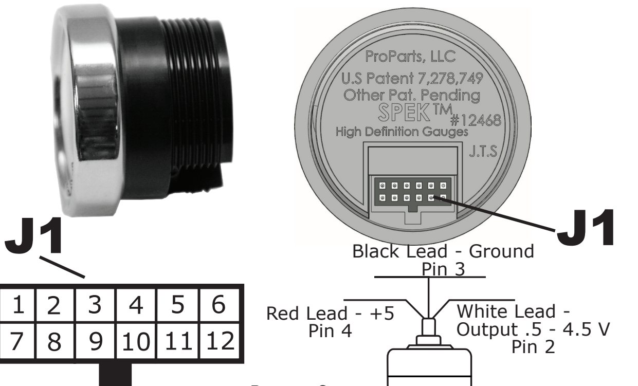
Pressure Sensor Wiring
