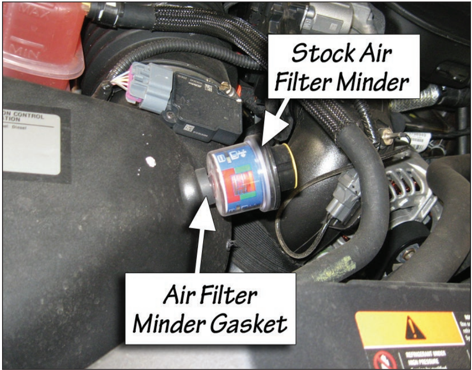
Figure 6- Remove Stock Air Filter Minder & Air Filter Minder Gasket
