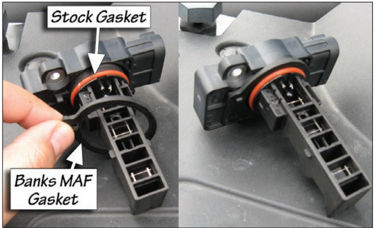
Figure 5a: Install Banks MAF Gasket
