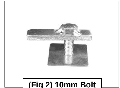
(Fig 2) 10mm Bolt Plate w-retainer
