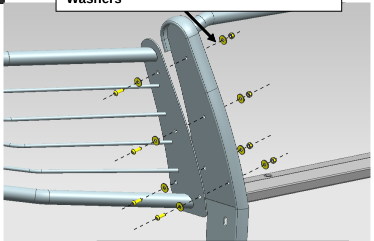
(Fig 12) Attach Right Brush Board to Middle Guard.
