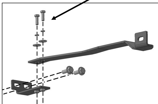
(Fig 10) Attach Top Support Bracket to top of Mounting Bracket
