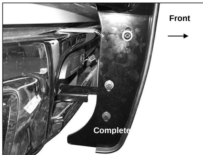
(Fig 14) Grille Guard attached to top and bottom Brackets
