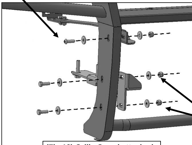
(Fig 13) Grille Guard attached to top and bottom Brackets
