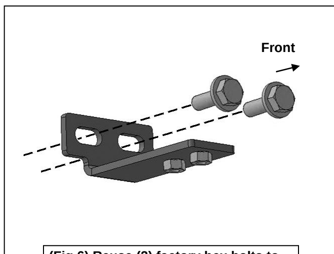
(Fig 6) Reuse (2) factory hex bolts to attach Top Support Mounting Bracket
