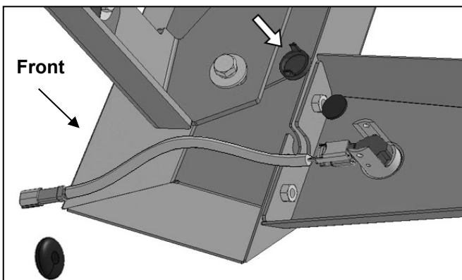
(Fig 17) Attach Sensor Plug into Sensor Sleeve
