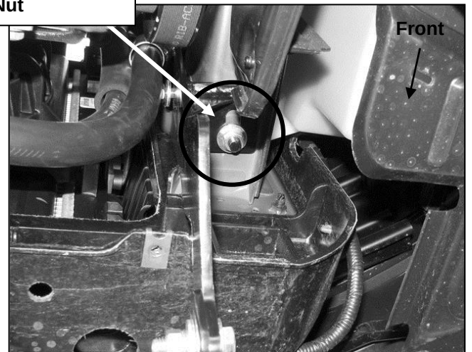
(Fig 7B) Bottom of passenger side Frame Bracket attached to Large Bolt Plate pictured from below
