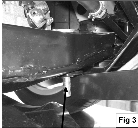
12mm x 90mm Bolt Plate
