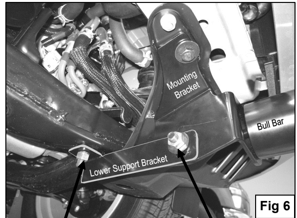
(12mm x 90mm Bolt Plate) 12mm Nylock Nut 12mm Flat Washer
