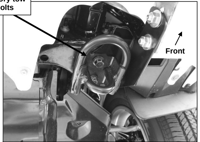
(Fig 4) Driver/left mounting Bracket installation
