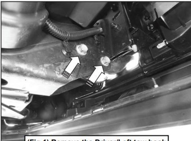
(Fig 1) Remove the Driver/Left tow hook
