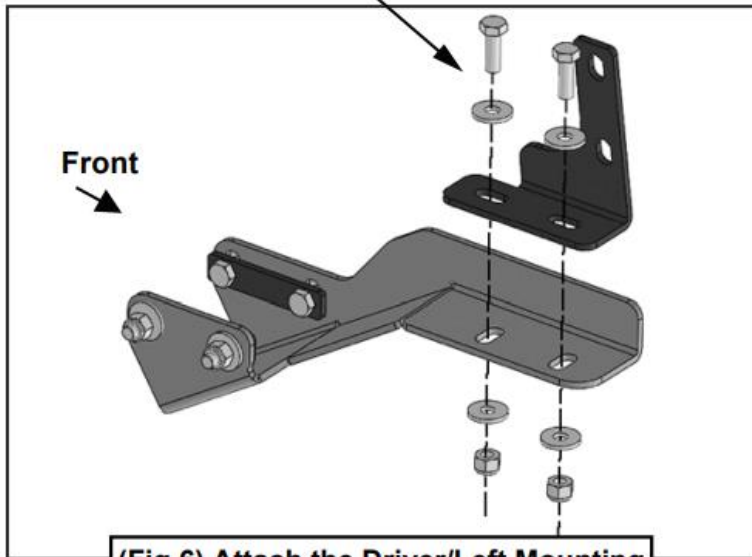
(Fig 6) Attach the Driver/Left Mounting Bracket to the Frame Bracket
