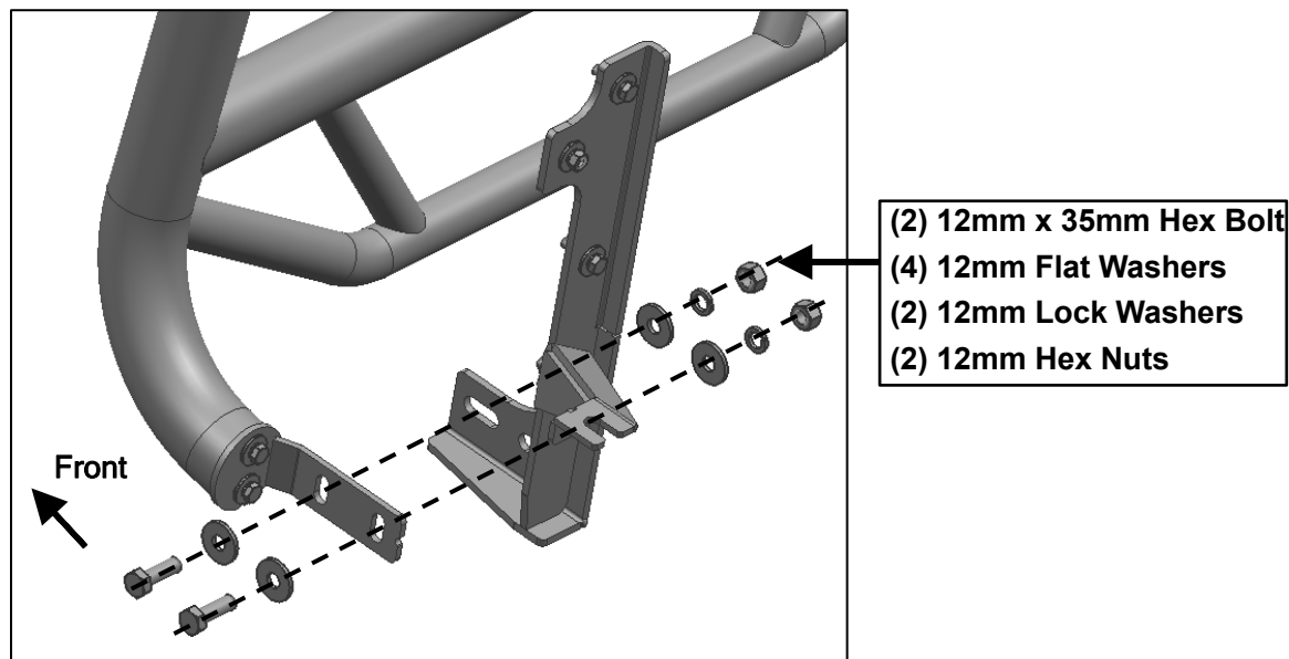
(Fig 7) Attach Guard to Mounting Brackets
