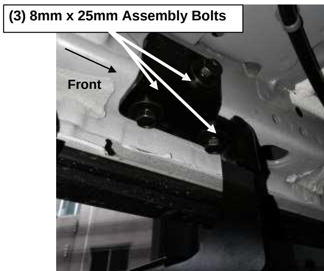
(Fig 5) Driver /Left Rear Mounting Bracket Pictured
