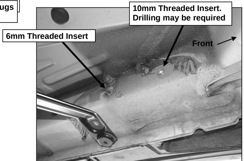
(Fig 4) Driver side front pictured
