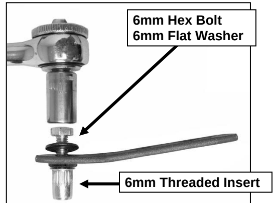
(Fig 2) 6mm Threaded Insert Tool assembly pictured
