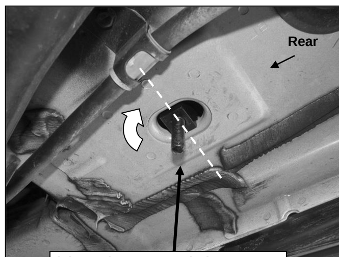
(Fig 15) Driver side rear mounting location
