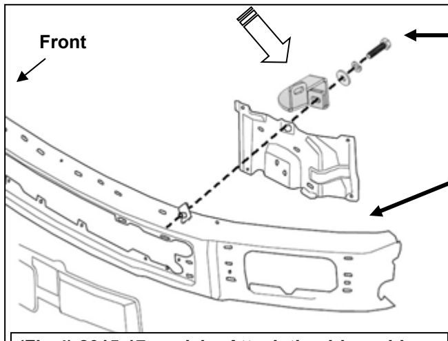
(Fig 4) 2015-17 models: Attach the driver side Top Bracket to the back of the middle mounting hole on the top of the bumper bracket
