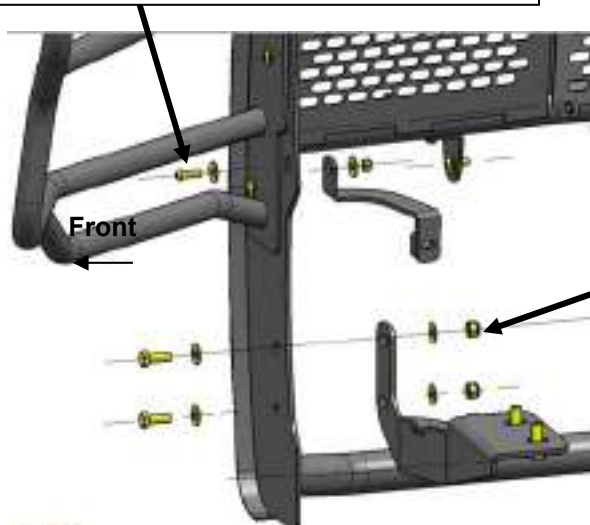
(Fig 24) 2015-17 models: Complete installation
