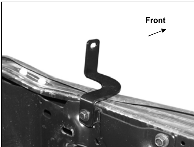
(Fig 21) 2018 models: Attach Top Support Bracket to back of bumper
