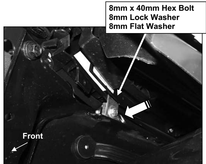
(Fig 5) 2015-17 models: Attach the driver side Top Bracket to the middle mounting hole on the top of the bumper bracket (pictured from behind bumper)
