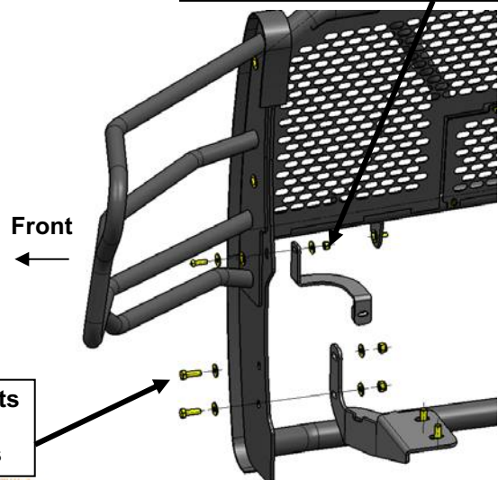
(Fig 25) 2018 models: Complete installation
