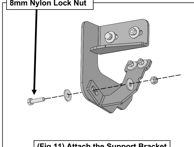
(Fig 11) Attach the Support Bracket to the Mounting Bracket
