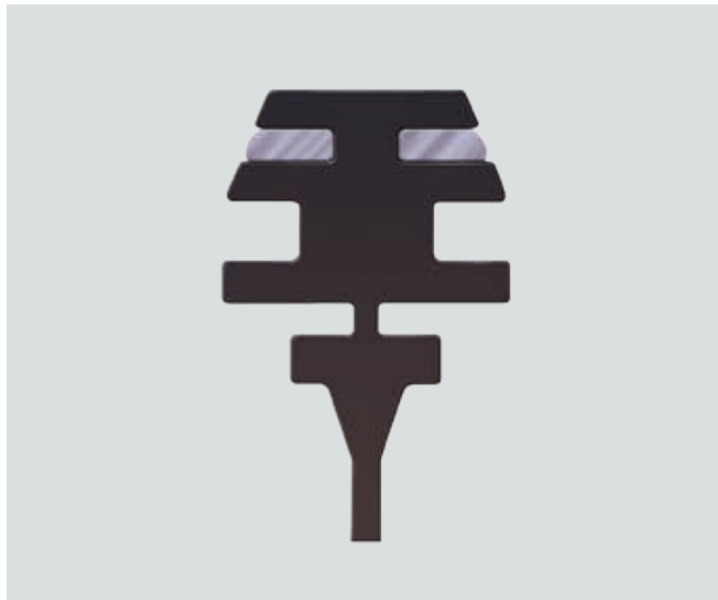
New Technology – External Metal Tension Springs
