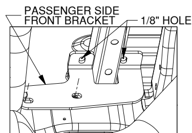
FIGURE A4: View looking up at the inside of passenger side frame.
