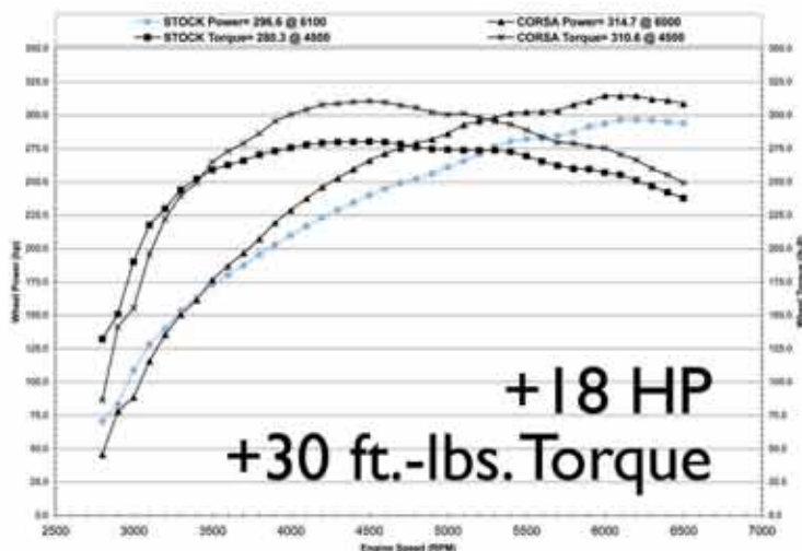
2006 CHEVROLET TRAILBLAZER SS 6.0L V8 - CHASSIS DYNO TESTING SAE Standard Corrected Data; Average Data of 3 Runs Each
