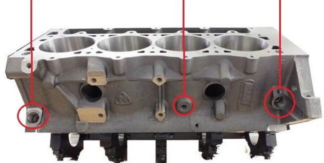
LS Next Drivers Side View
