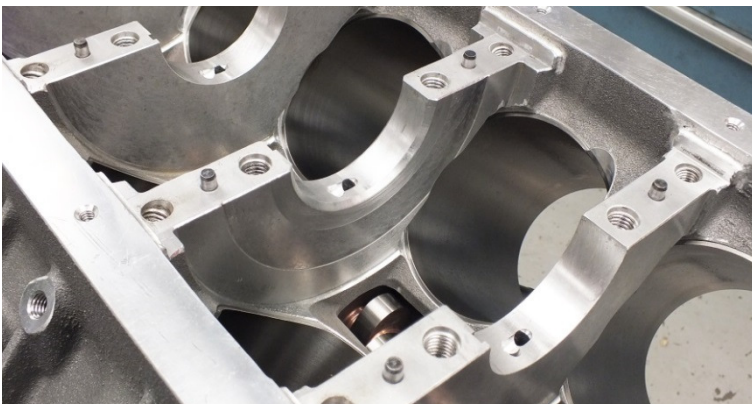
LS Next 2 Blocks come machined with clearance
