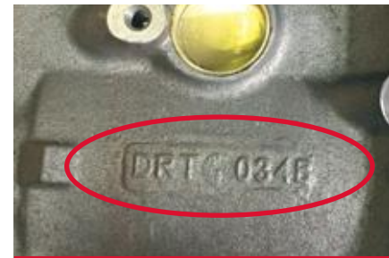
MRK IV, Gen V and Gen VI blocks with water between the bores are identified by a B suffix on the casting number.
