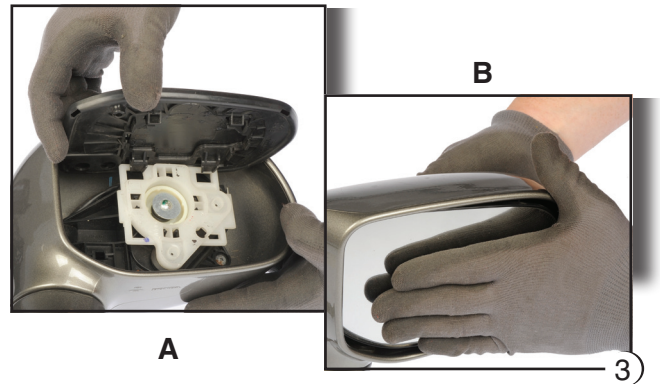
Fig. 3 A-B. Installing your new mirror glass assembly.
