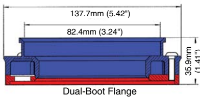
Dual-Boot Flange
