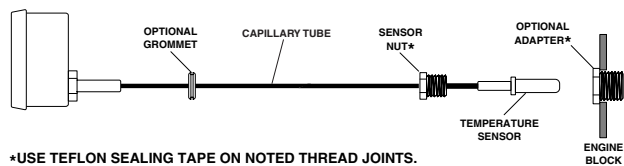
Figure 6. Mechanical Water Temperature Gauge Connections
