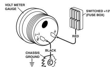
Figure 4. Voltmeter Connections
