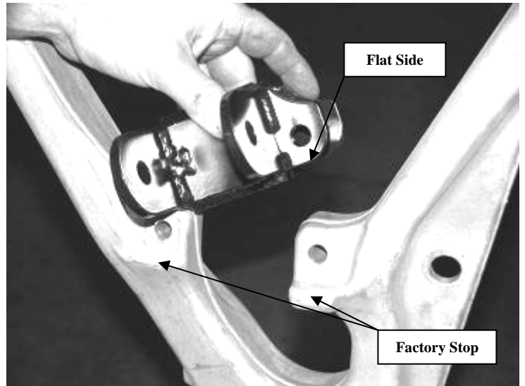
20. Locate FT20339 Lower Shock Mount, FT20352 Lower Mount Shim, and the supplied 7/16" x 2 1/2" hardware. Position the mount onto the lower control arm so the flat side of the bracket will be flush with the stop on the arm. Position the shim in between the new mount and the control arm. Attach with the 7/16" hardware and torque to 50 ft lbs. Rotate the lower control arm up and attach the strut to the new mount with the provided 1/2" x 3 3/4" hardware and torque to 75 ft lbs. (it may be necessary to rotate the shock and extension to attach). Torque the top shock bolts to 40 ft lbs. SEE PHOTOS BELOW AND ON NEXT PAGE.
