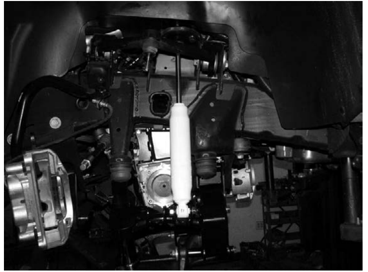
40. Locate the factory crossmember the torsion bar runs through. This cross member will need a small amount of clearance added to it. At the intersection of the frame and the crossmember, grind a 2" Radius 1/4" deep. SEE PHOTO BELOW
