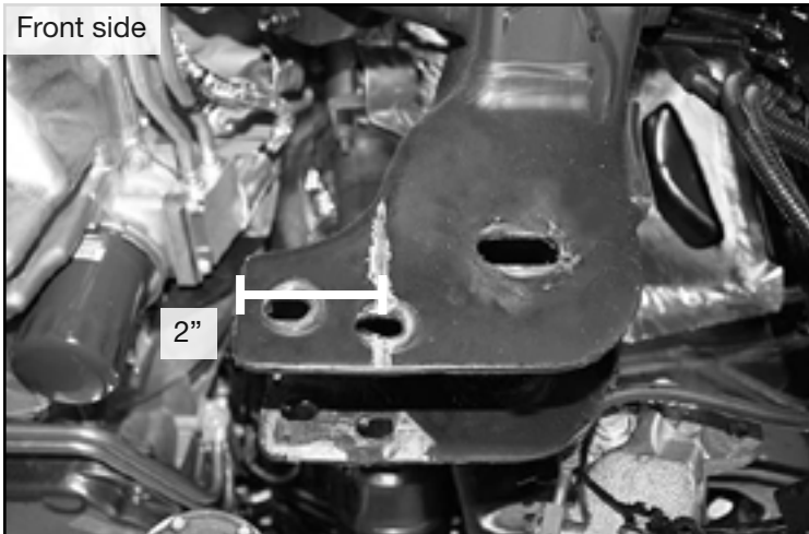
FIGURE 29 - STEP 20
