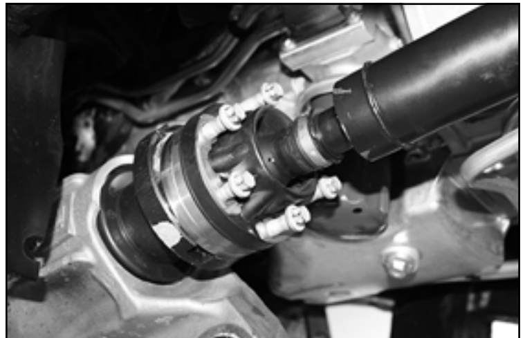
FIGURE 43 - STEP 27
