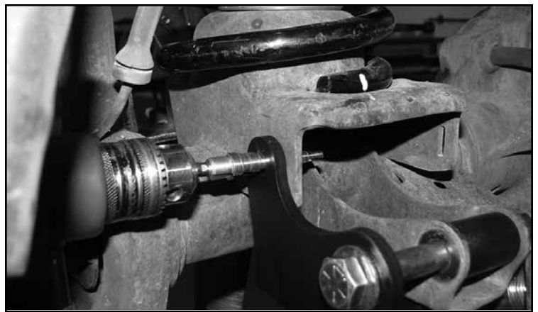
FIGURE 16 - STEP 12
