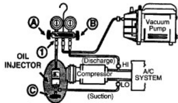
ADDING OIL OR CONDITIONER TO DISCHARGED SYSTEM
