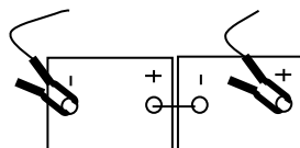
2- 12V batteries in series: add \frac{1}{2} rated capacities of single battery. Pack is 24V.
