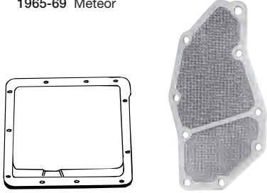
Pan has 11 holes
