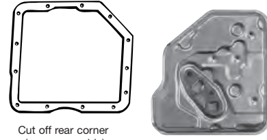
Pan has 13 holes
