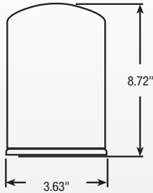
8.72" (H) x 3.63" (OD) Filter
