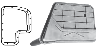
Pan has 15 holes
