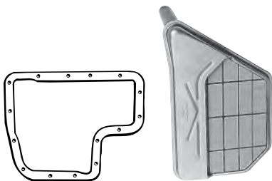
Pan has 15 holes
