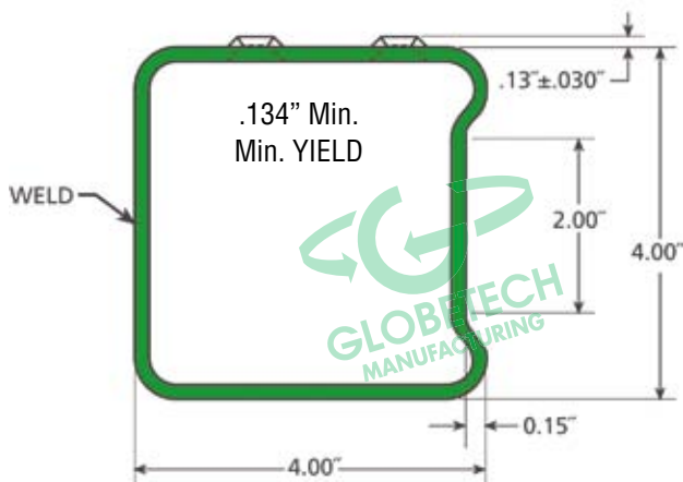
Cross Section
