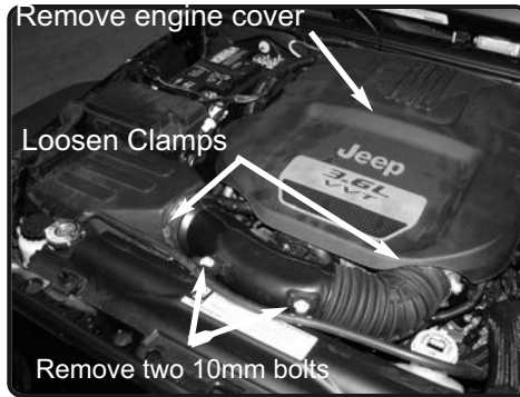
2. Lift up firmly to remove the engine cover. Continue to loosen the two clamps from the throttle body and air duct. Then remove the two 10mm bolts pictured.
