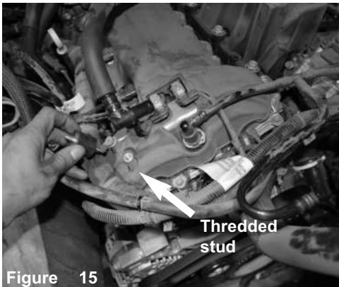
Figure 15 Locate the threaded stud on engine. With provided M6 vibramount, secure to the engine.
