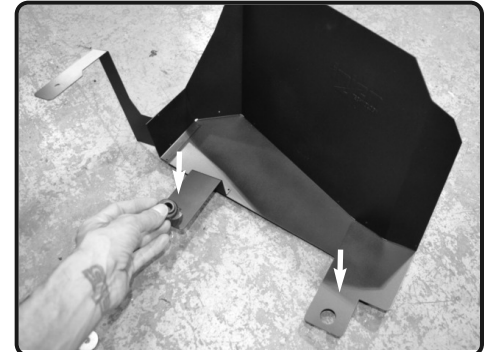
7. Install the provided 2 6014 grommets to the holes on the heatshield.
