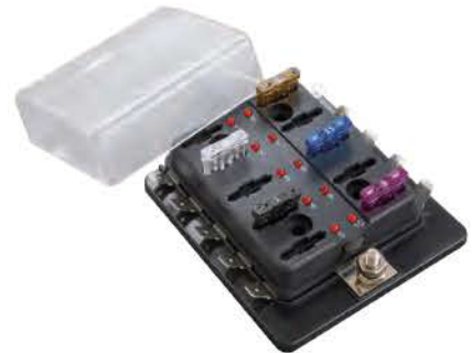
LED ATC FUSE BLOCKS BLR-I-310 10-POSITION FUSE BLOCK WITH INDICATING LEDS. FOR USE WITH REGULAR AUTO BLADE FUSES. EA
