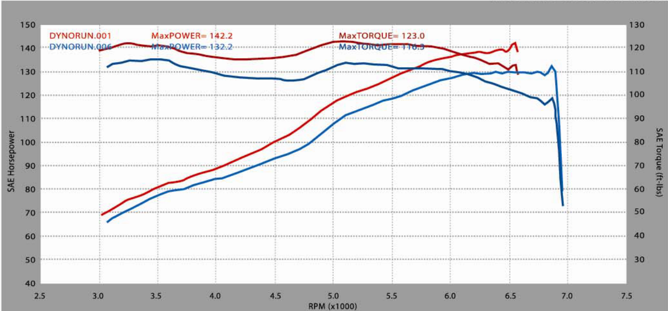
HONDA 02-UP CIVIC EP3 SI EXHAUST
