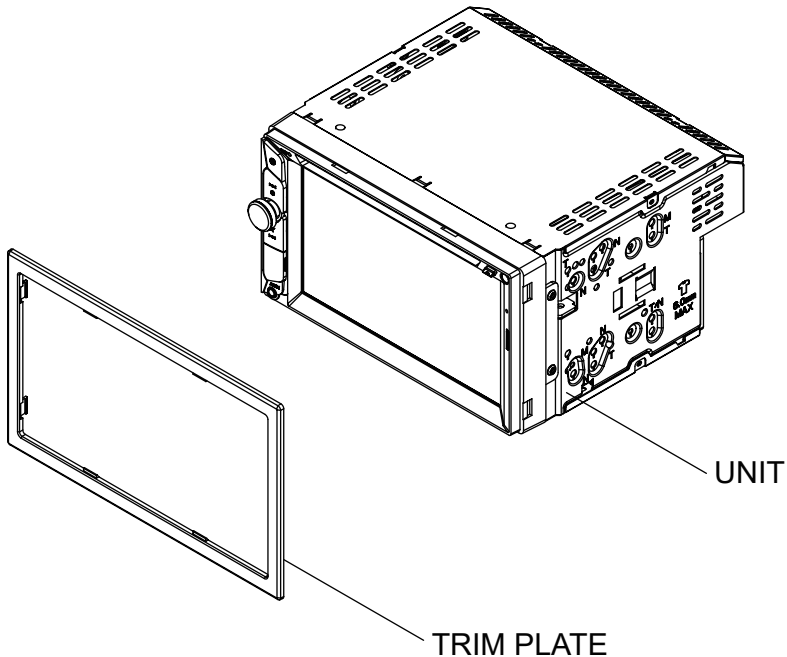
TYPICAL FRONT-LOAD DIN MOUNTING METHOD
