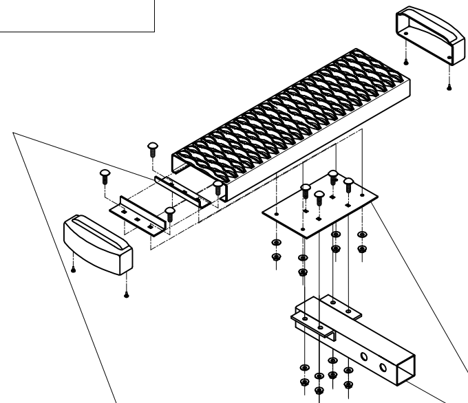
STINGER-PKG (570010)
