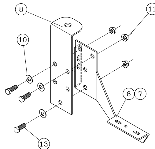
CREW CAB REAR BRACKET ASSEMBLY
