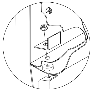
PINCH WELD SUPPORT ASSEMBLE
