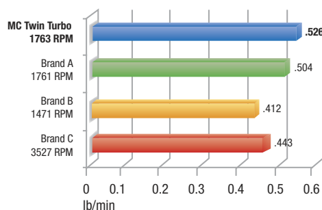
Vapor Recovery (ln) lb/min • Temperature: 79 to 82°F / Refrigerant: R134a
