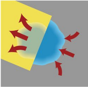
self absorptivity
