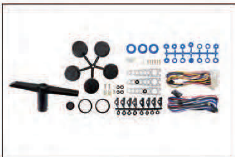
PROW-2002 UNIVERSAL POWER WINDOWS • with 3 switches (2 window power window kit) • Complete kit to convert 2 manual windows to full power • Power window system • Installed behind the door panel • Cuprum bearing • POM plastic gear wheel
