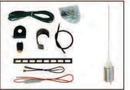
PRO-1070 TRUNK RELEASE ACTUATOR • Operating voltage: 12V DC • Operating temp.: -30 deg. C - +70 deg. C • Weight: 200g
