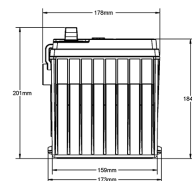
ODX-AGM34/78 LEFT POSITIVE DUAL TERMINALS (SAE & SIDE)
