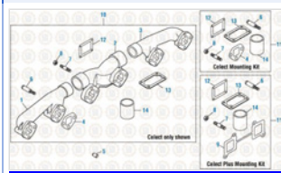
Cummins Engine 2017 Exhaust Manifold - N14 Series
